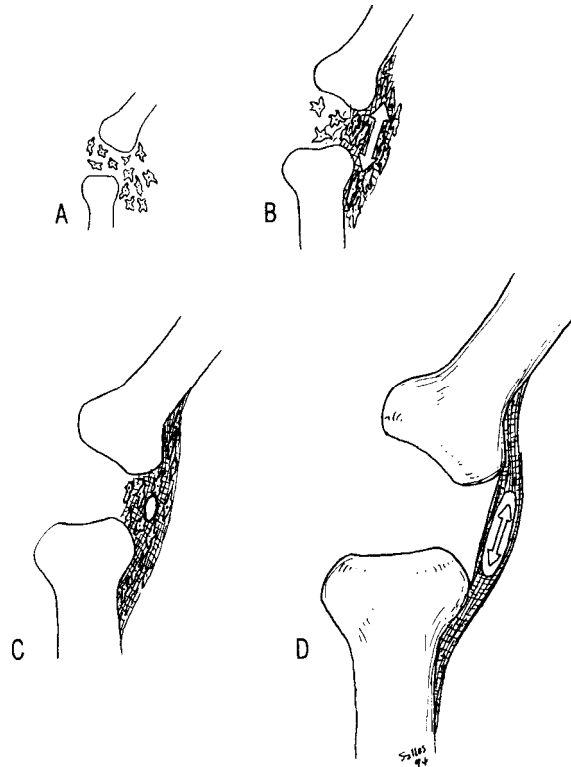
Figure 2-4 Tendon/ligament formation.
